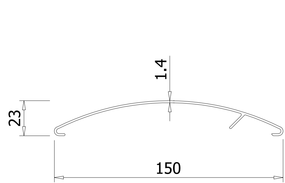
ASC P150 profile
